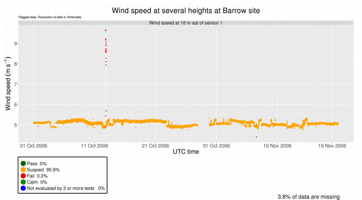
Figure 8. Wind speed time series at 18 meters above ground level at Barrow site, USA ( 71.32^{\circ}\text{N} 156.61^{\circ}\text{W} , 11 m)
