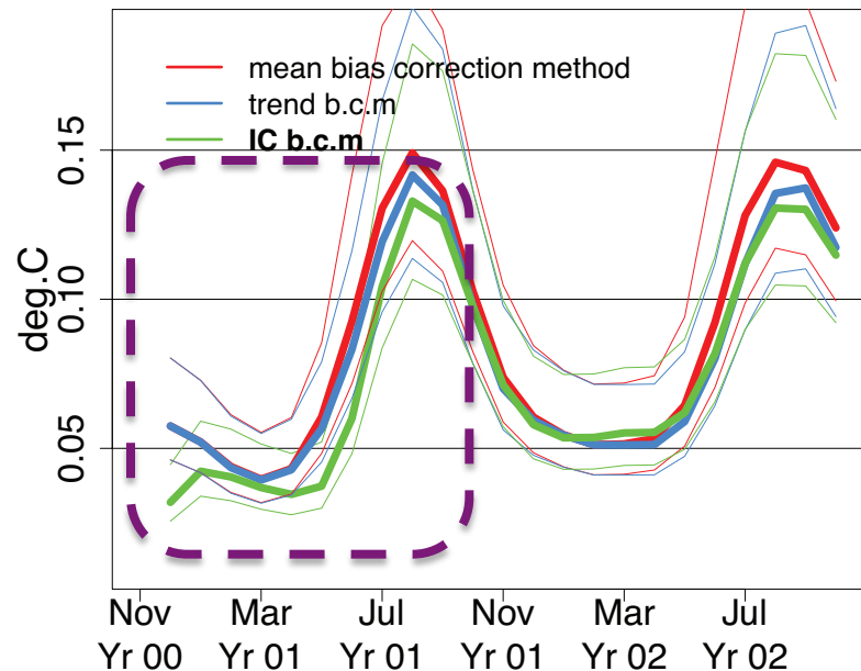
3-month smoothed RMSE of SST north of 60°N
