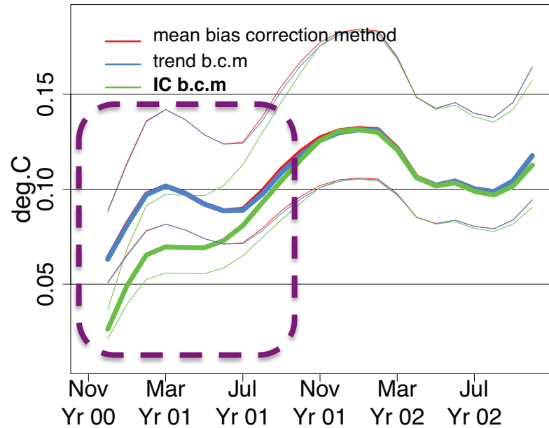
3-month smoothed RMSE of tropical SST
