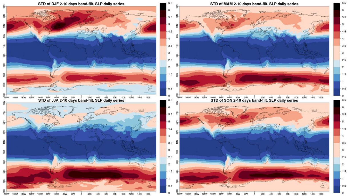
Figure 2. Standard deviation of the 2-to-10 day bandpass filtered ERA-Interm data.
