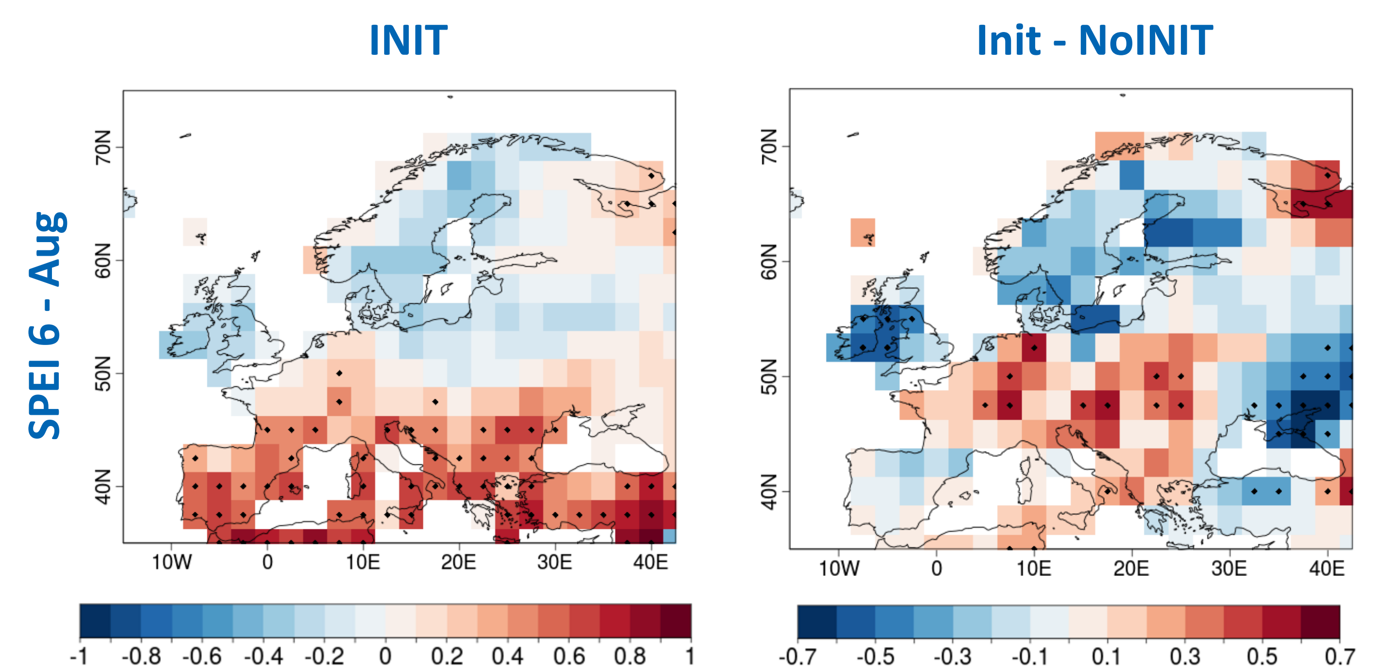
Figure 5: Ensemble mean correlation map of SPEI6 (August) averaged over the forecast years 2 to 5 (left column: initialized prediction, right column: difference between INIT and No-INIT simulation). Dotted region – statistically significant at 95% confidence level
