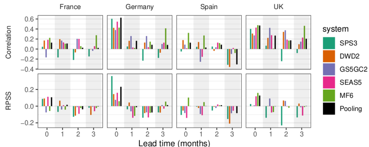
Fig 3. Skill assessment of energy forecasts that combine the teleconnection predictions and their observed impacts.
