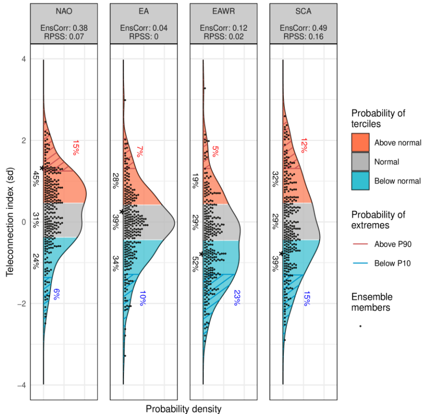
Fig 1. Probabilistic seasonal forecasts of four teleconnection indices from C3S.
