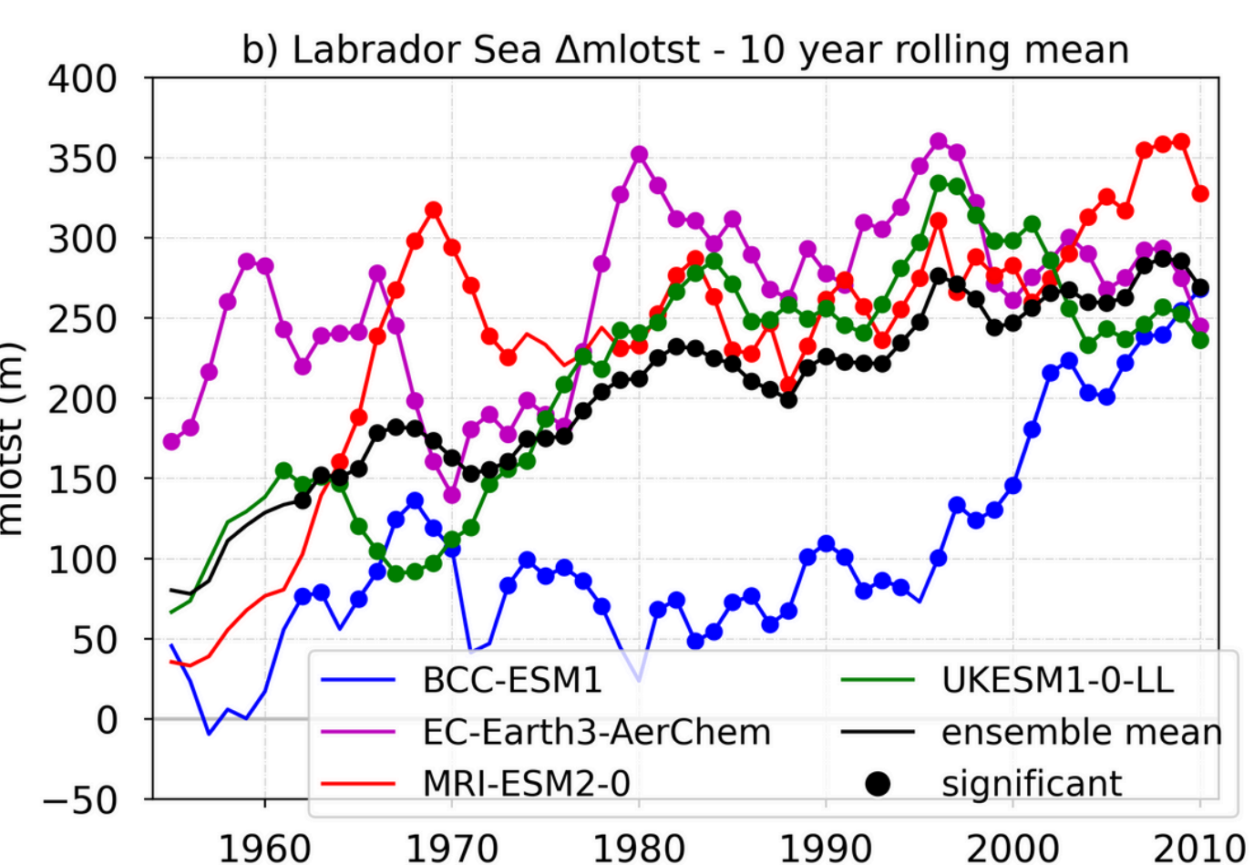
NTCF signal on mixed layer depth in the (a) North Atlantic and (b) Labrador Sea
