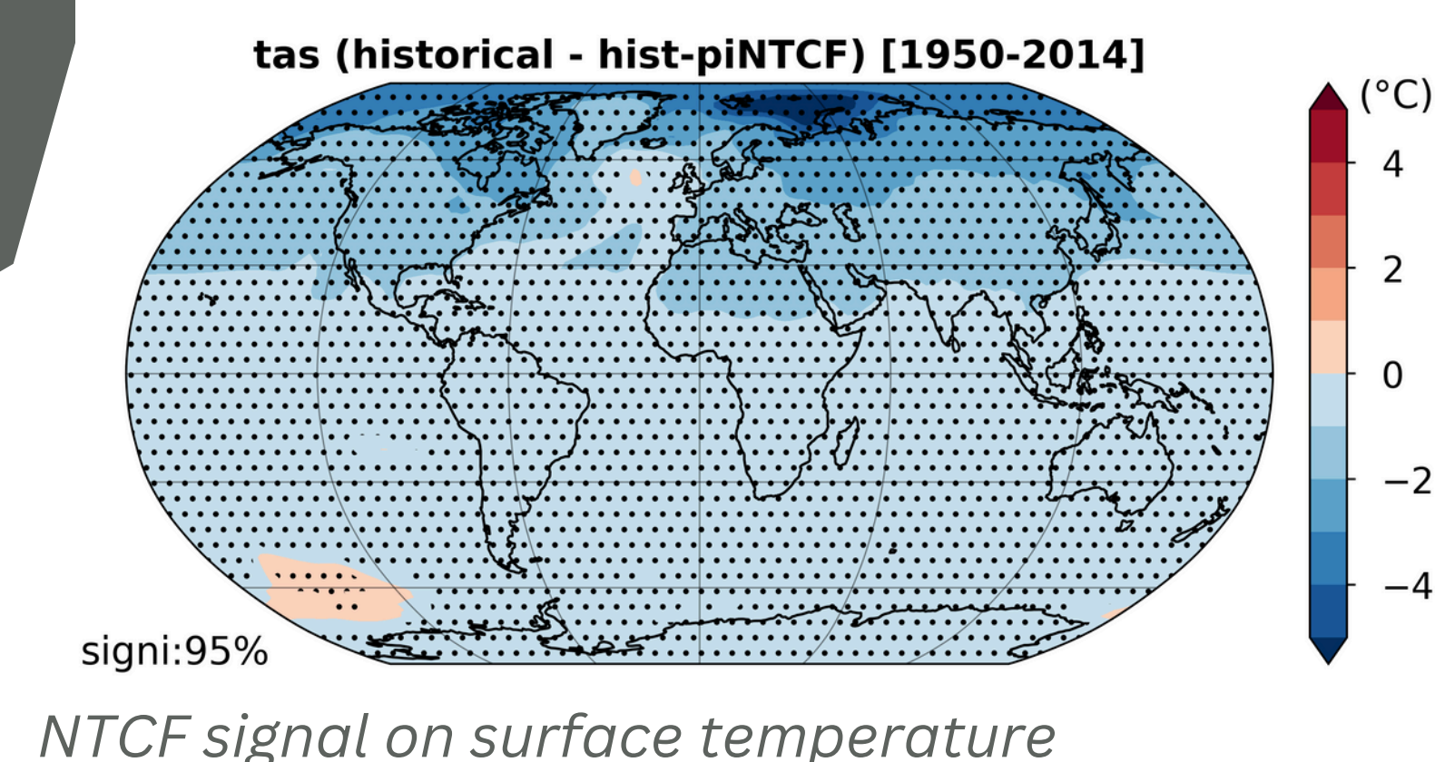
NTCF signal on surface temperature
