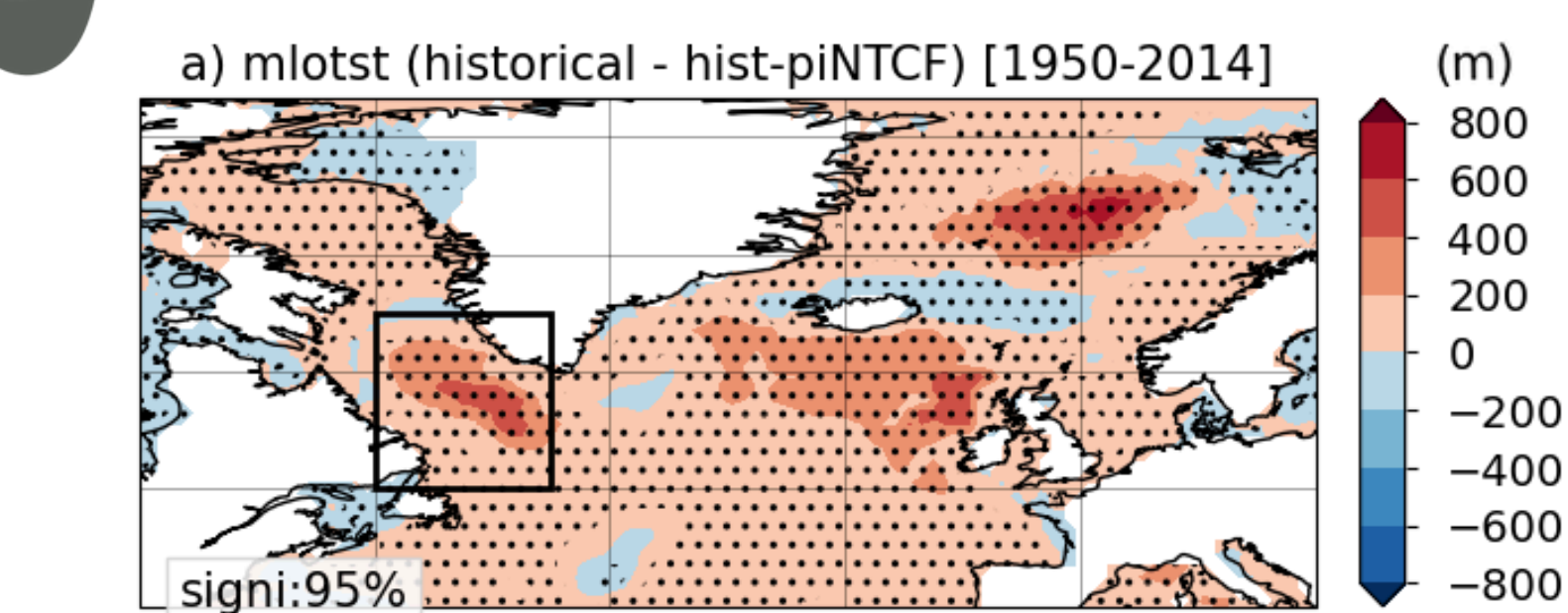
NTCF signal on mixed layer depth in the (a) North Atlantic and (b) Labrador Sea
