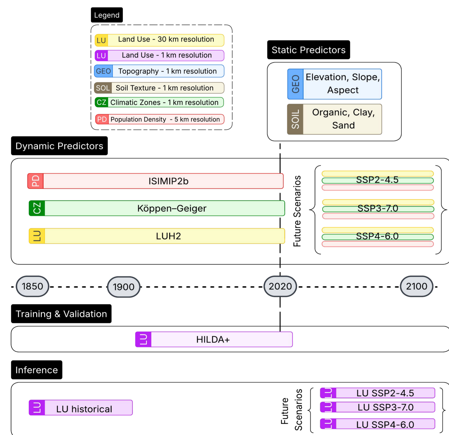
Figure 1: Temporal coverage of the framework's data. This includes the dynamic predictors (population ISIMIP2b, climatic zones Köppen-Geiger, and 30 km land use LUH2h), static predictors (elevation GEBCO, topography and soil PNNL), high-resolution training target (1 km land use HILDA+), and final inferred 1 km LU output for 1850-2100.
