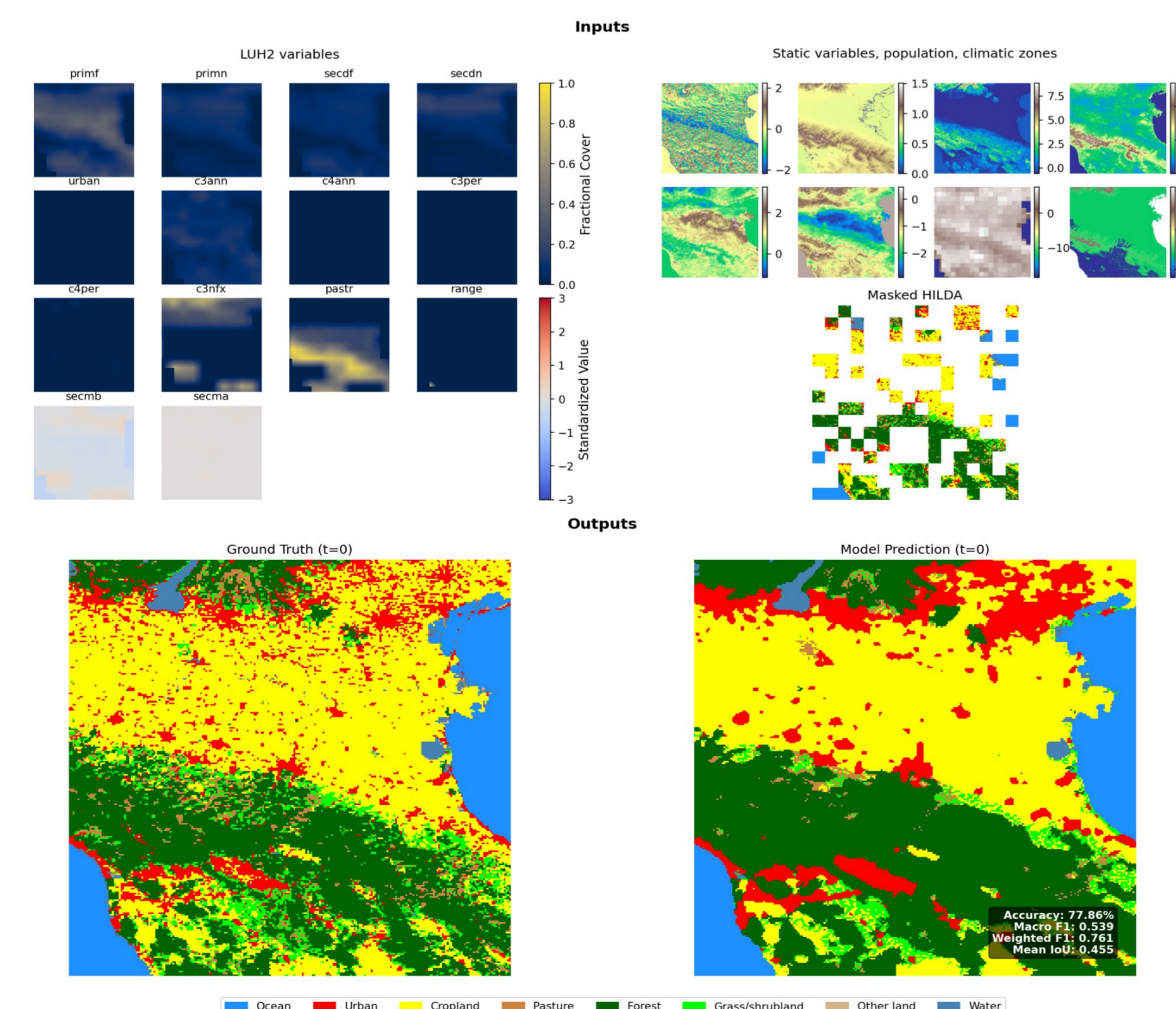
Figure 2: Overview of the LU reconstruction pipeline for Bologna, year 2014. The U-Net model combines coarse-resolution LU, population, climatic zones, elevation, soil, and a masked high-resolution prior LU to predict the final high-resolution LU output.
