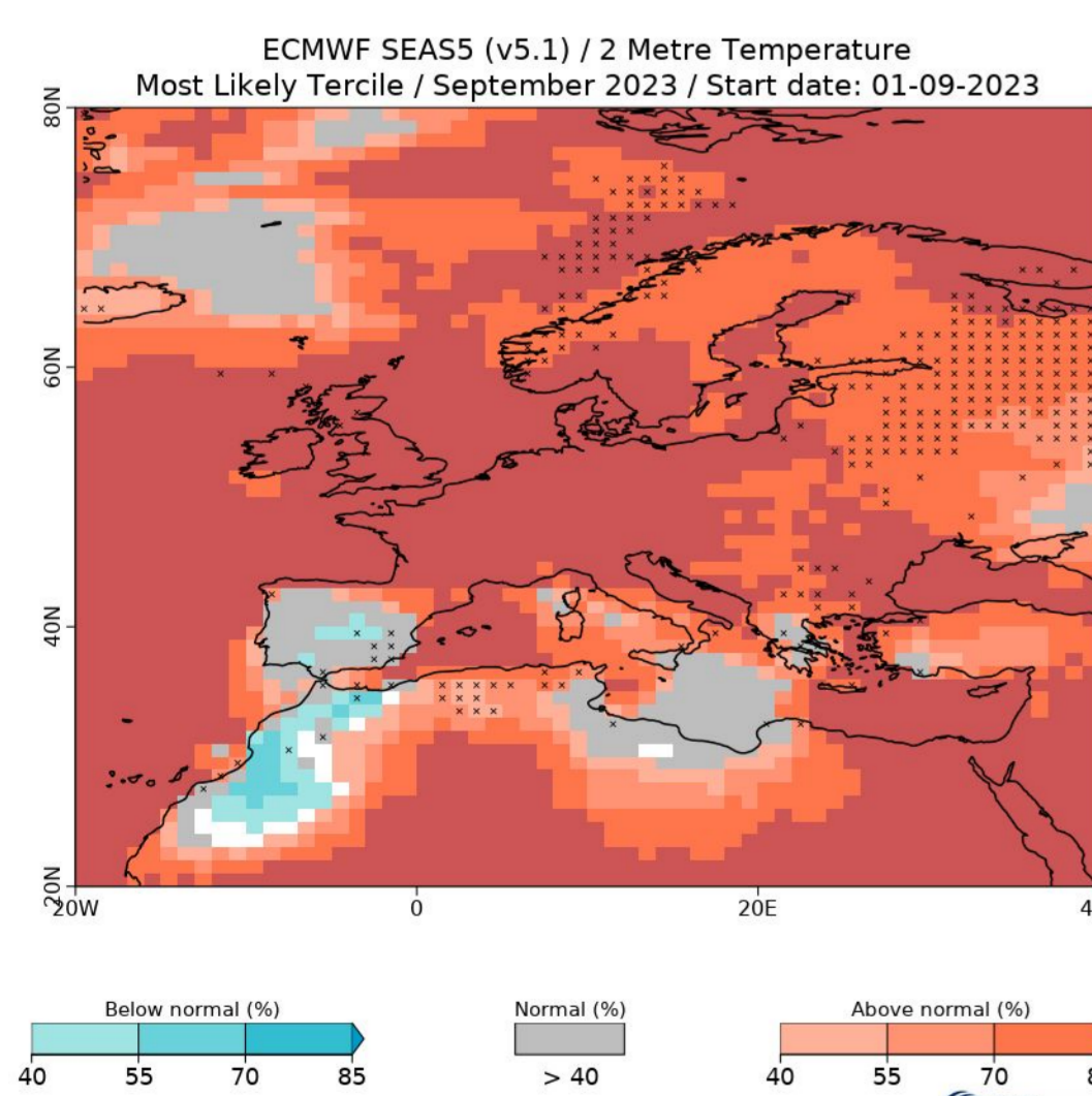
Fig 5: Most-likely terciles for September 2023 2 metre temperature, for the ECMWF SEAS5 (v5.1) September-initialized forecast. Crosses indicate grid points with negative Rank Probability Skill Score (RPSS).
