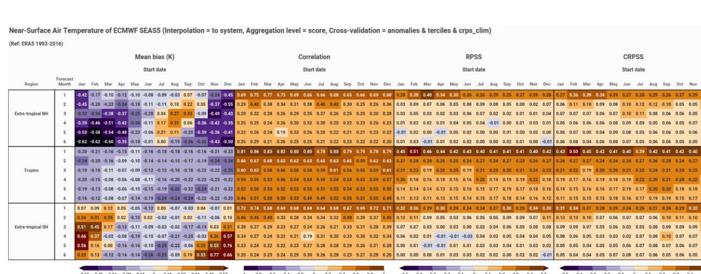
Fig 7: Scorecard displaying the near-surface air temperature mean bias, correlation, RPSS and continuous rank probability skill score (CRPSS) values for the 1993-2016 hindcast period in three regions (tropics and extra-tropics) for each initialization date of ECMWF SEAS5, computed using ERA5 as the reference dataset. The user can decide which metrics and regions to display in the scorecard.
