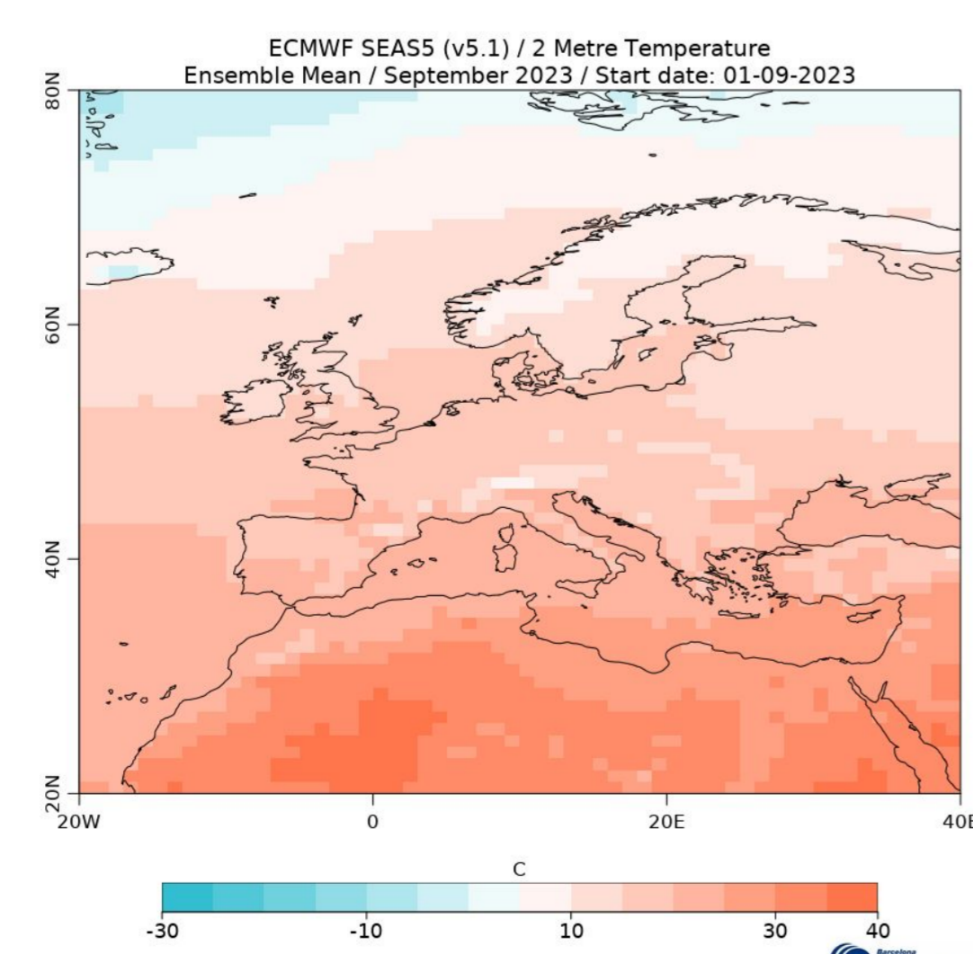
Fig 6: Forecast ensemble mean for September 2023 2 metre temperature, for the ECMWF SEAS5 (v5.1) September-initialized forecast.
