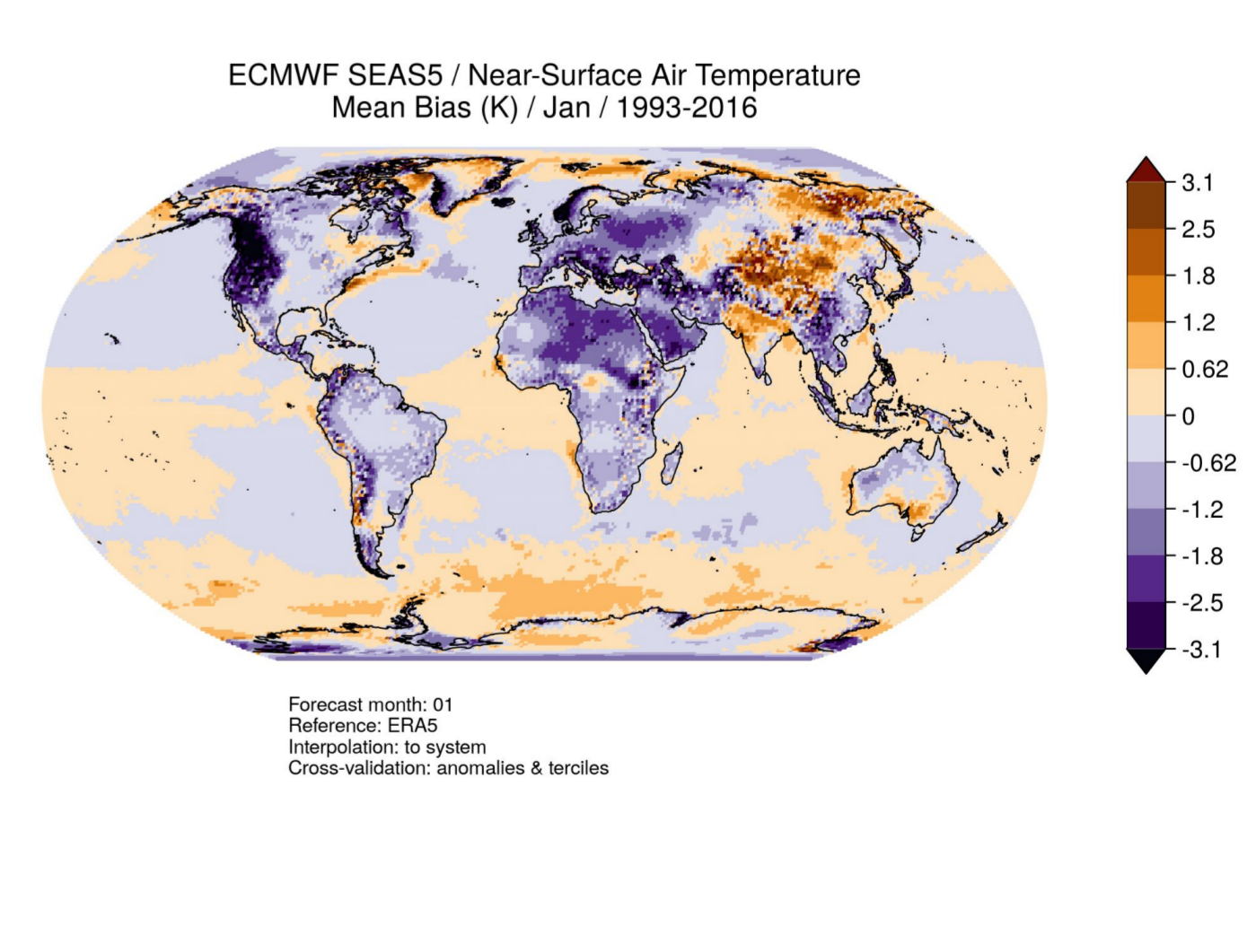
Fig 8: Robinson projection map, showing the mean bias of January near-surface air temperature for ECMWF SEAS5 evaluated against ERA5 for the 1993-2016 hindcast period, initialized in January.
