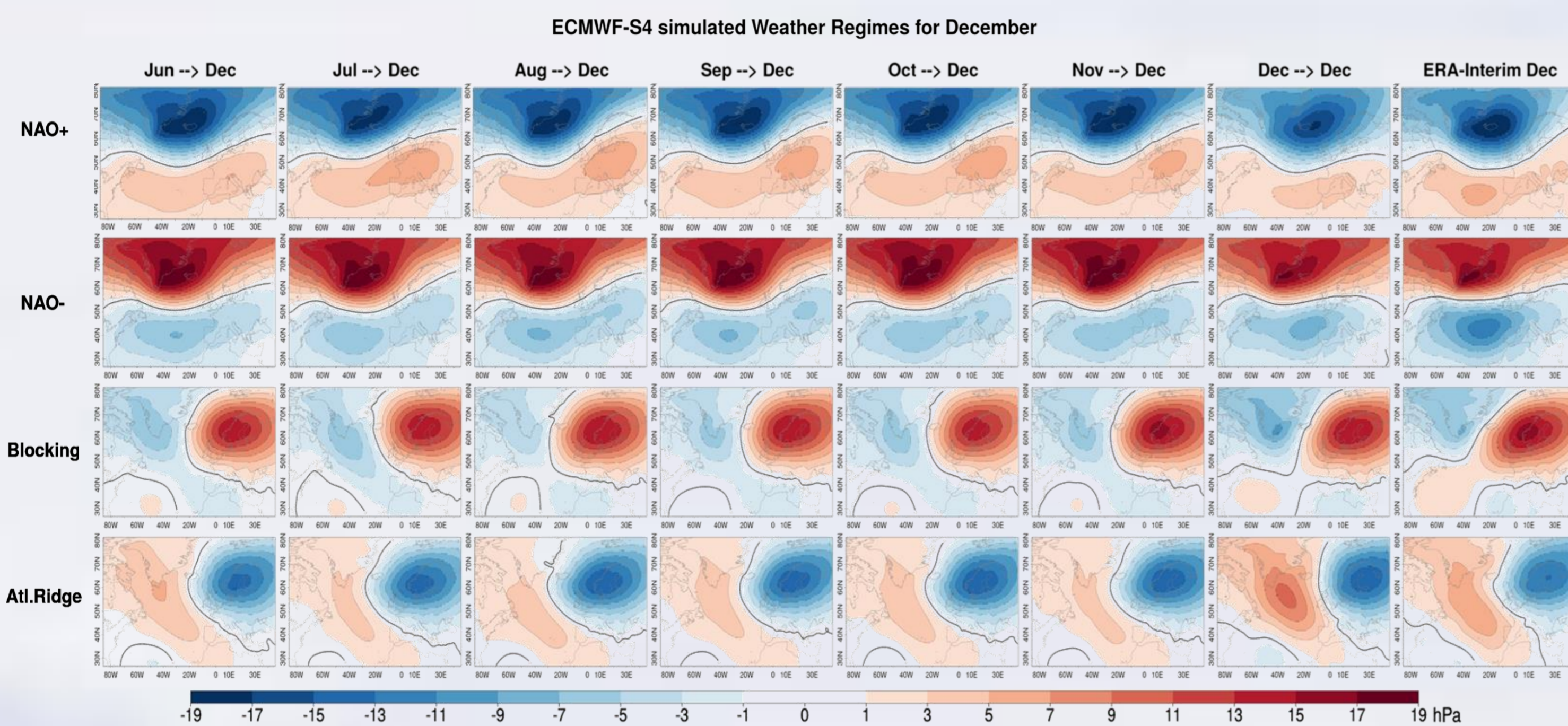
Figure 1. S4 simulated regime anomalies (in hPa) for the target month of December (1981-2015) and different startdates and lead times (from 6 to 0 months) vs ERA-Interim observed regime anomalies (last column to the right). Black lines show null anomalies.
