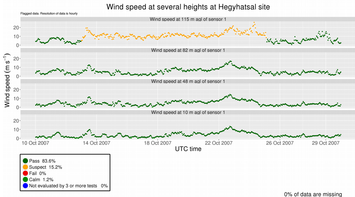
Figure 12. Wind speed time series at 10, 48, 82 and 115 meters above ground level at Hegyhatsal tall tower, Hungary (46.96° N, 16.65° E, 248 m).
