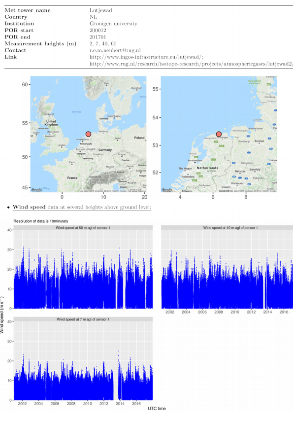
Figure 5. Summary sheet for a meteorological mast at Lutjewad, the Netherlands (53.40° N, 6.35° E, 60 m).
