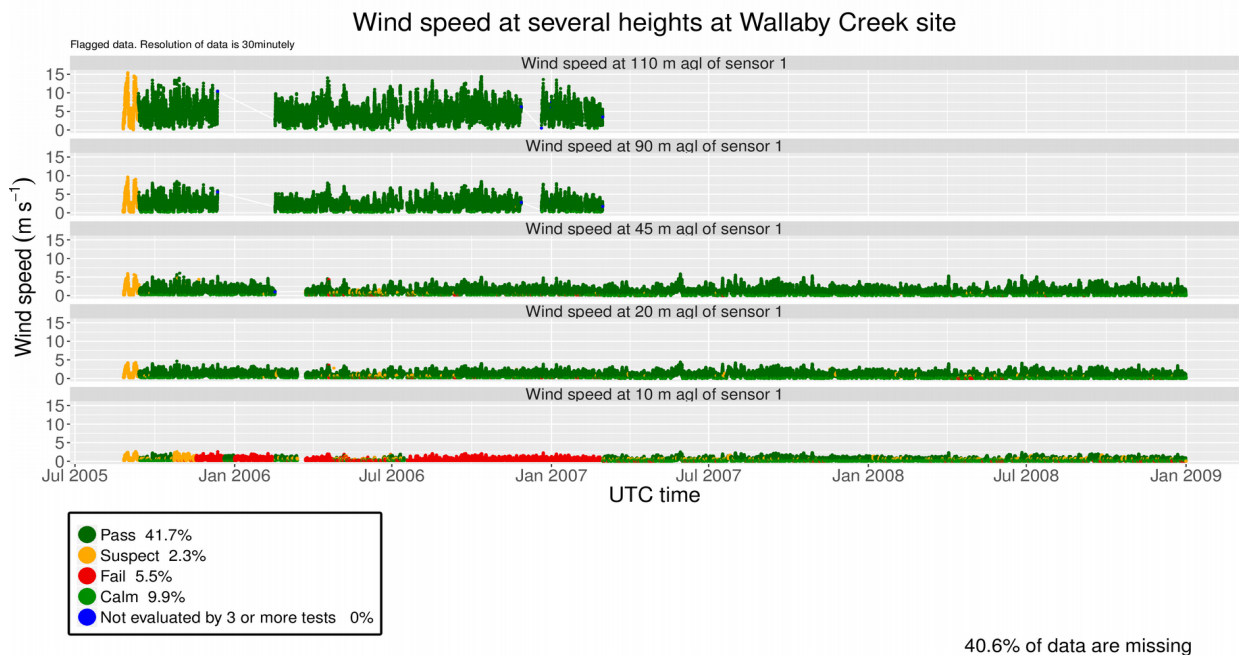
Figure 7. Wind speeds at 10, 20, 45, 90 and 110 meters above ground level at Wallaby Creek site, Australia ( 37.42^\circ \text{ S} , 145.19^\circ \text{ E} , 720 m).
