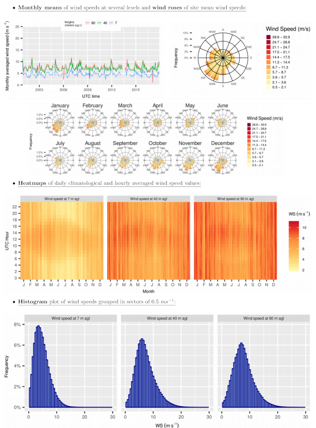
Figure 5. Summary sheet for a meteorological mast at Lutjewad, the Netherlands (53.40° N, 6.35° E, 60 m).
